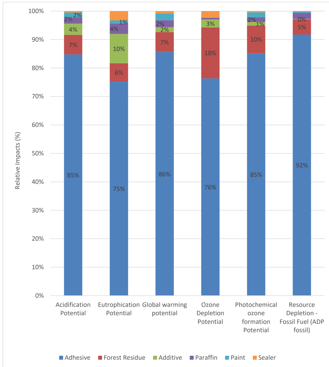
Figure 5: Contribution analysis of materials in module A1 for CanExel.
