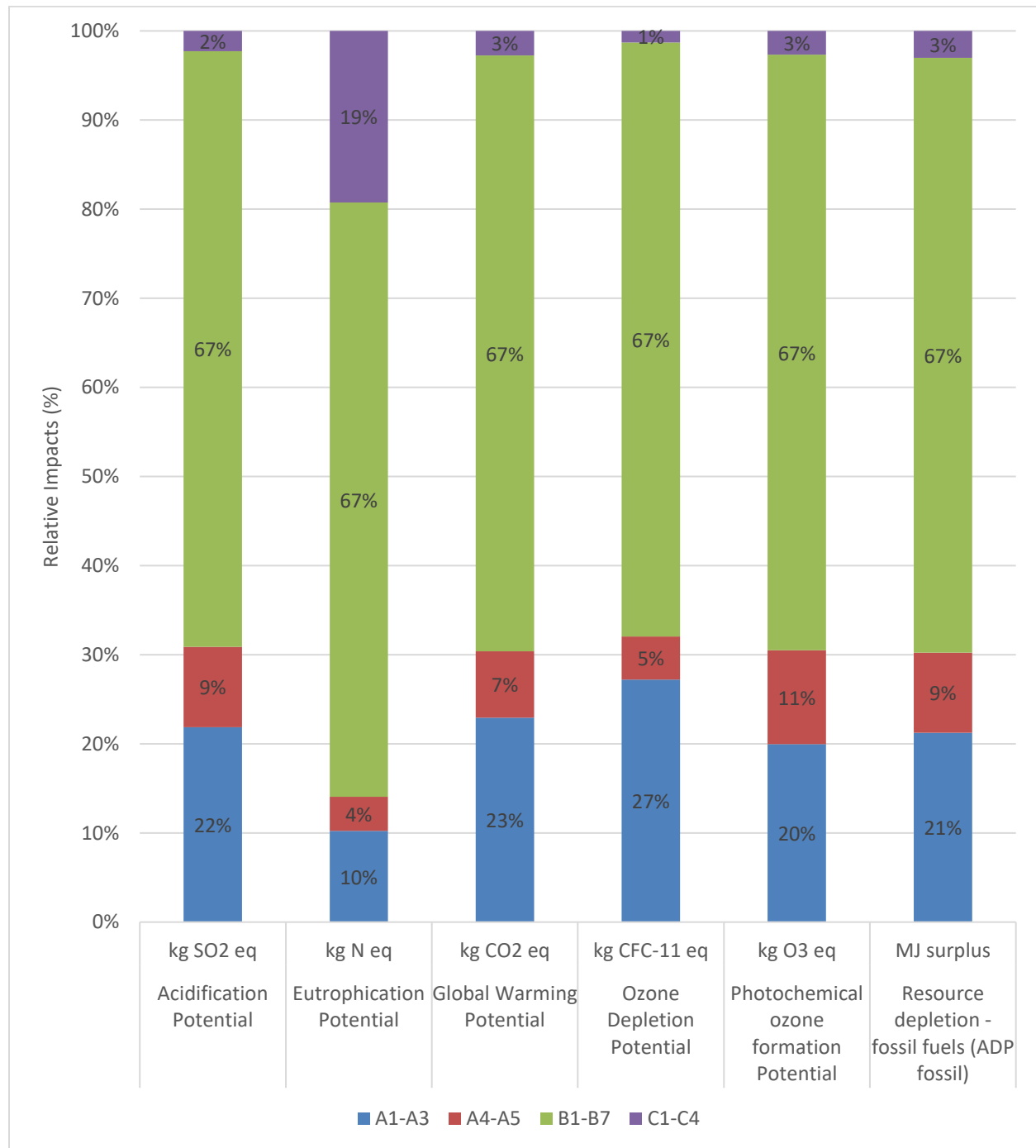
Figure 3: Contribution of each life cycle stage for CanExel.
