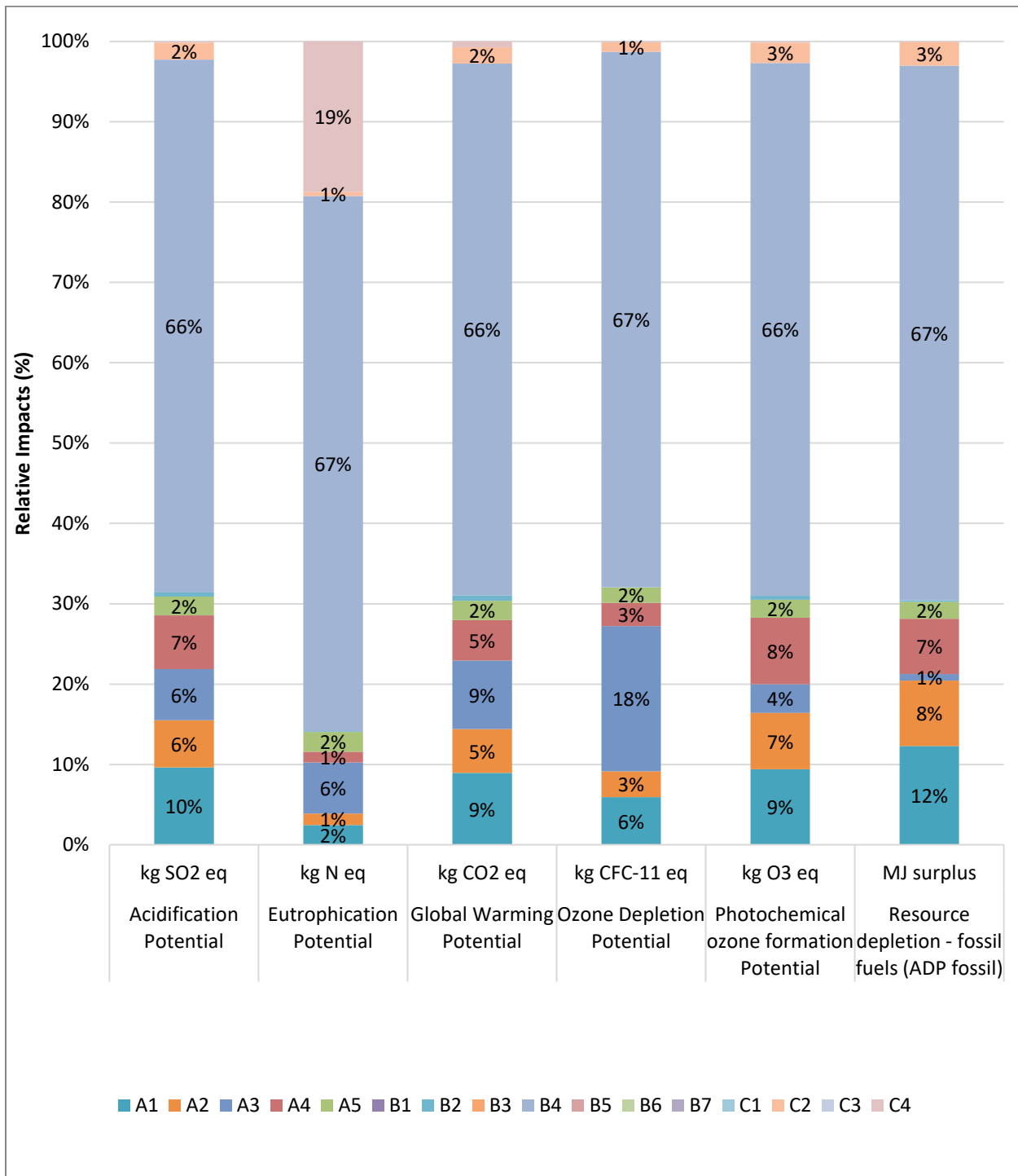
Figure 4: Contribution of each life cycle module for CanExel.
