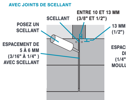
FIGURE 2 PLANCHE - PLANCHE
