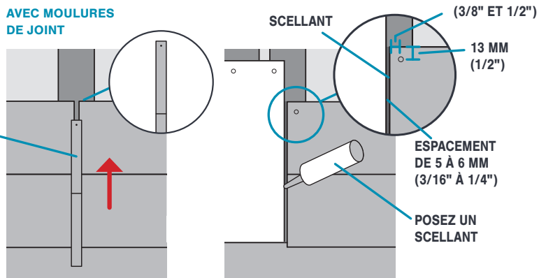
FIGURE 3 PLANCHE - MOULURE
