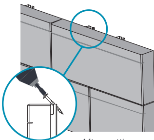
FASTEN SCREW AT AN ANGLE
