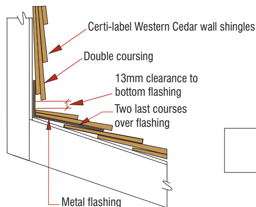
Figure 3a: Flashing
